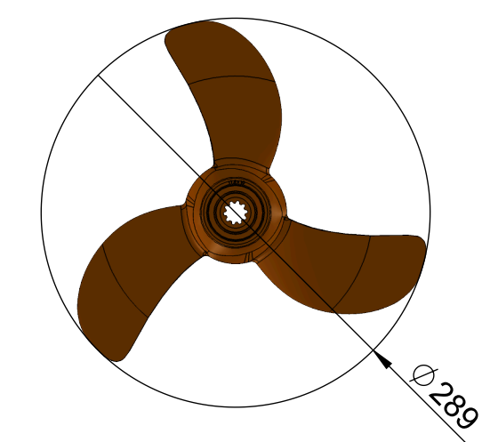
Cruise 3.0 Standard Propeller B 11,5x10 WDR [1996-00]
