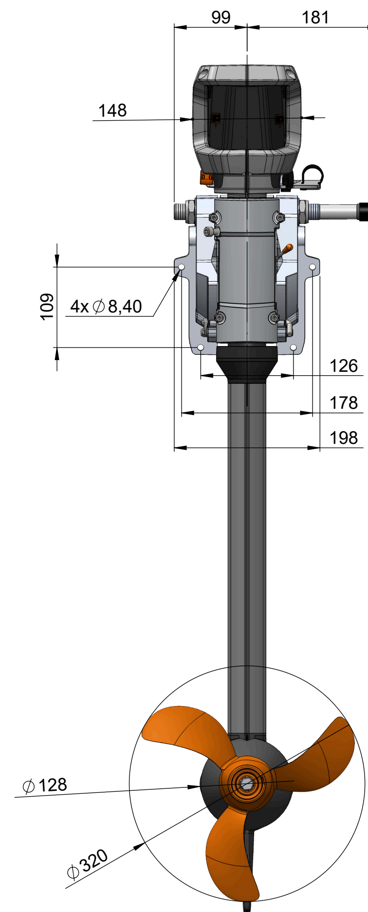
Cruise 6.0 Standard Propeller B 12,5x17 HSP [1987-00]
